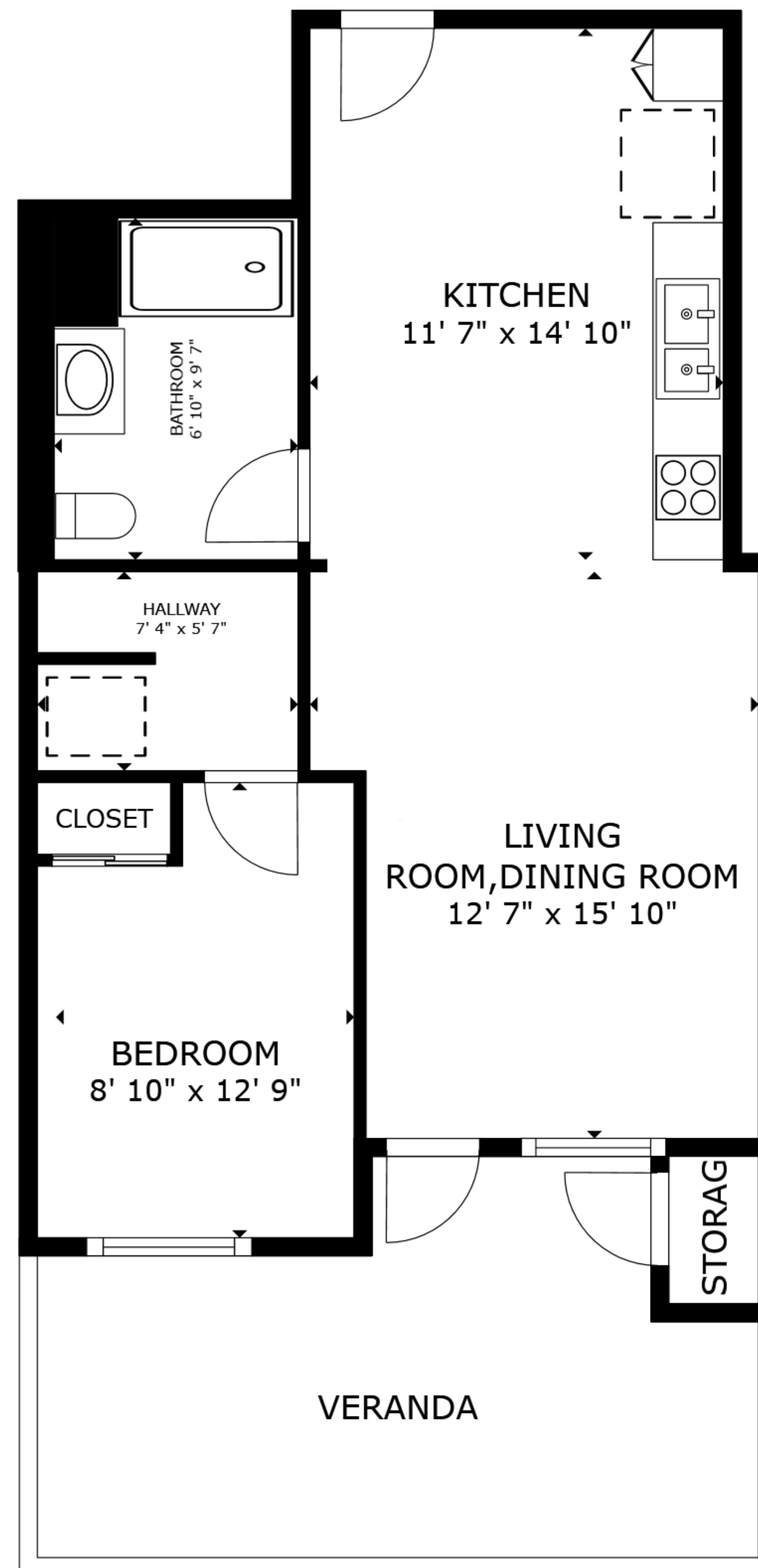
FLOOR PLAN
